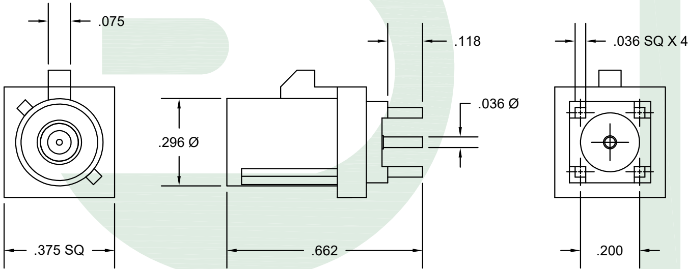
FAKRA CONNECTOR CODE C
