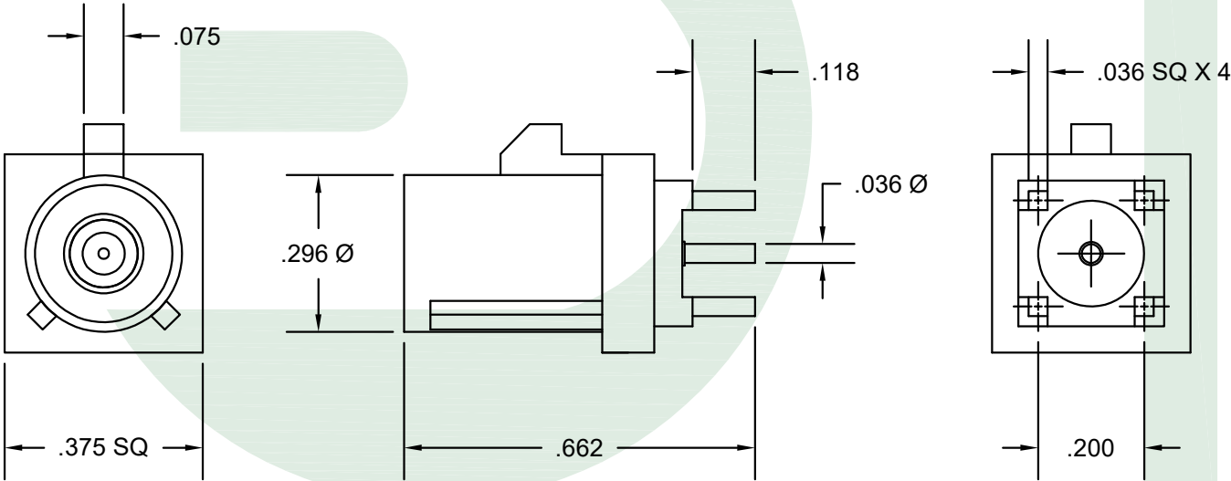
FAKRA CONNECTOR CODE K
