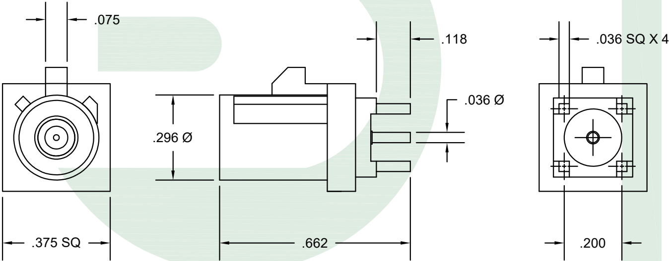
FAKRA CONNECTOR CODE B
