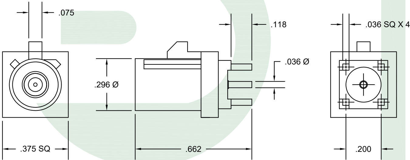
FAKRA CONNECTOR CODE A
