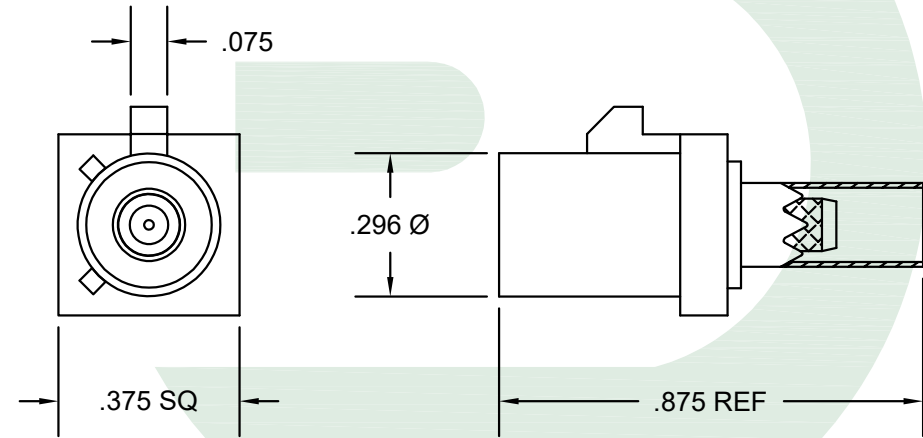
FAKRA CONNECTOR CODE D
