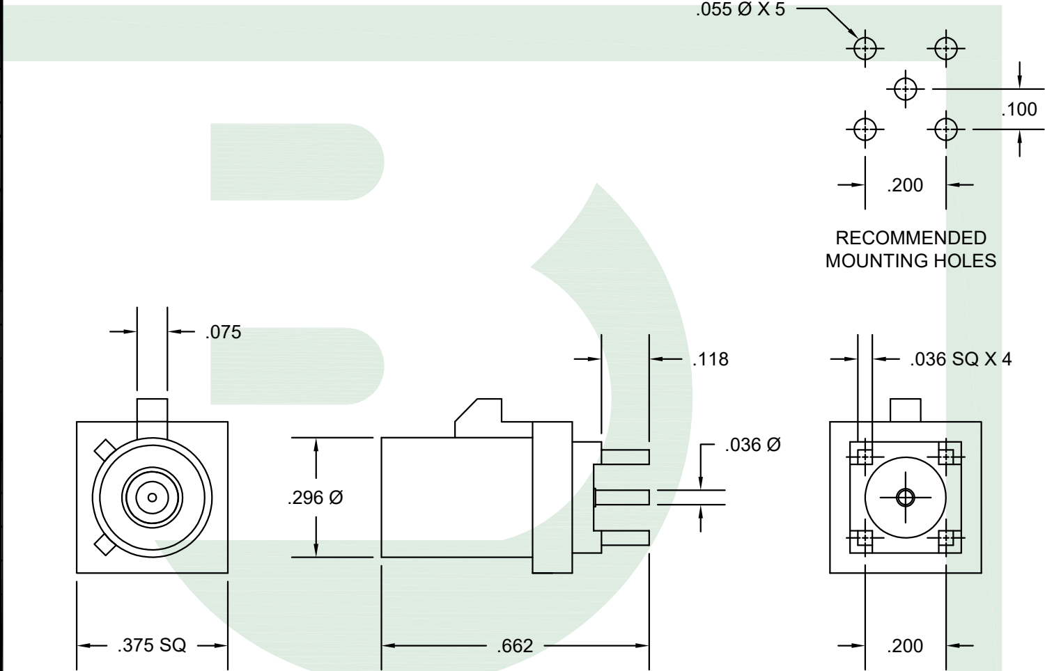
FAKRA CONNECTOR CODE D
